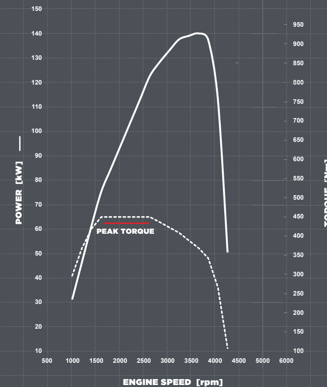
C Engine Performance Curve
